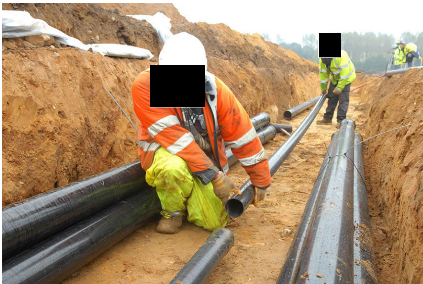
Plate 4-20: Example of hand laying ducts within open trench (Source: Equinor)
